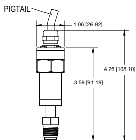
VCR SWIVEL MALE PIGTAIL GFDXXXXPSMA FITTING A333124001 ME131193
